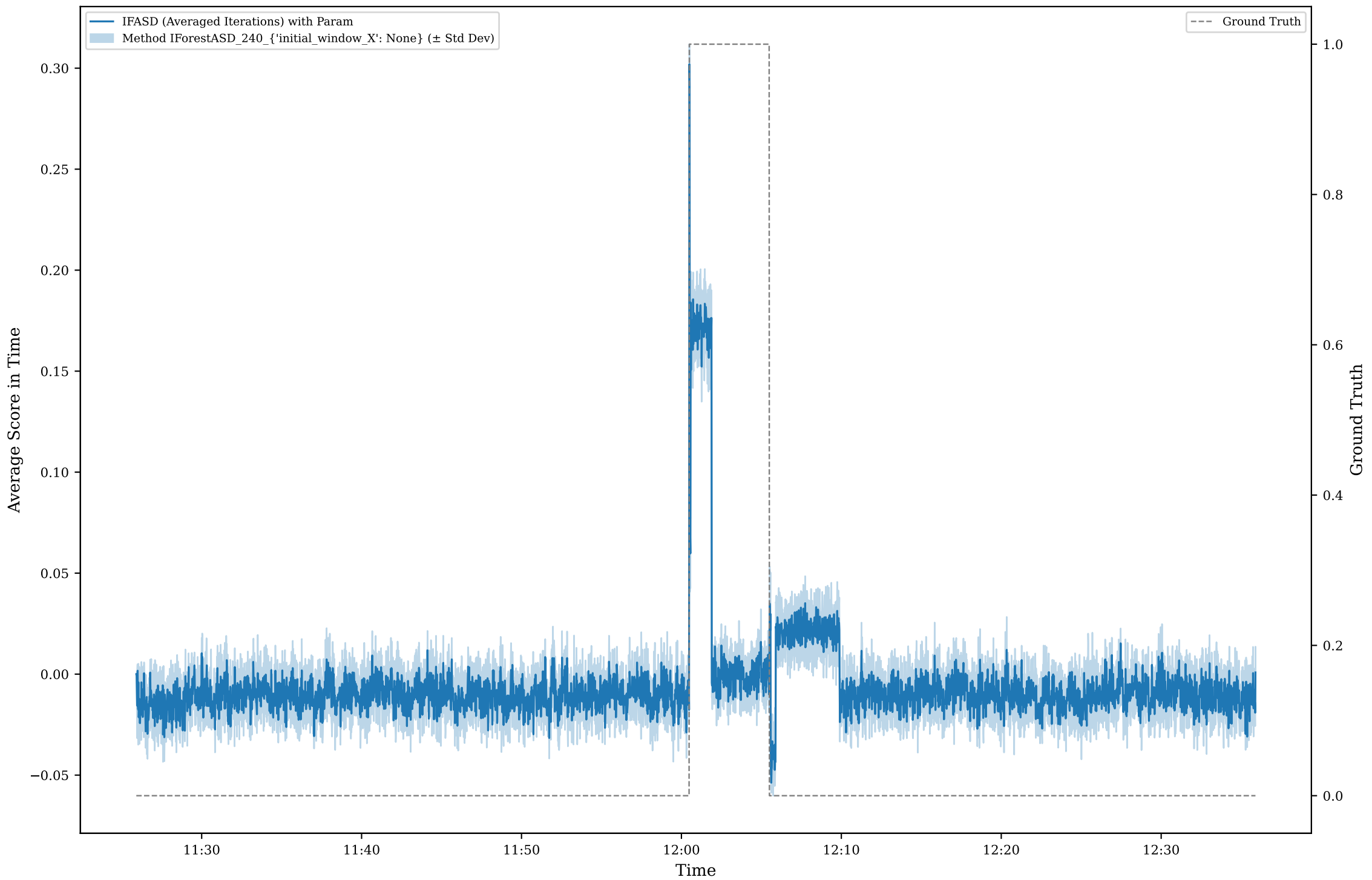
Method IFASD Score for Scenario A5
